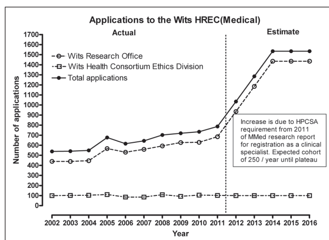
Fig. 6. Comparison of WRO and estimated WHCED new applications including the anticipated WRO application load due to new HPCSA policy.
