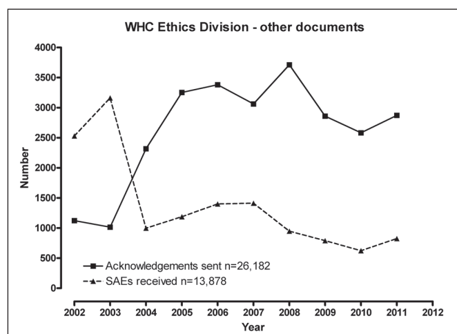
Fig. 4. X-Y plots for the frequency of 'other documents' by year.
