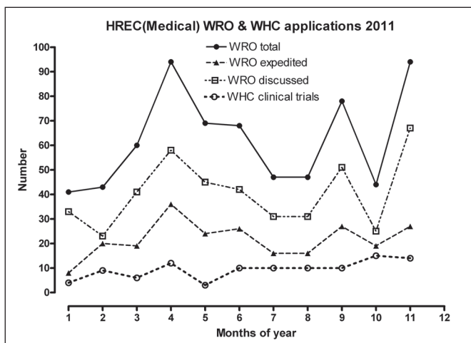
Fig. 2. Pattern of applications by month in 2011.
