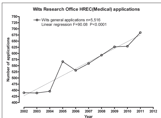
Fig. 1. X-Y plot of new general research applications by year.
