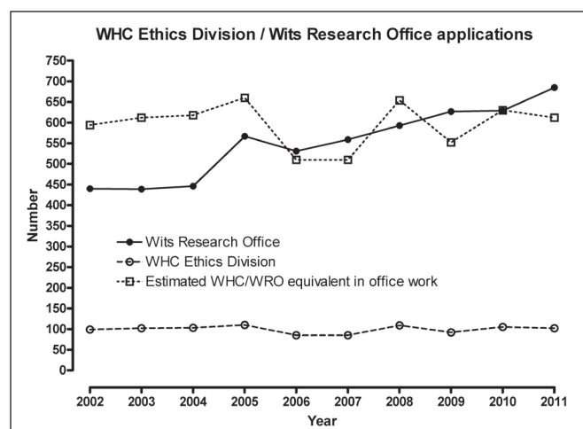
Fig. 5. Comparison of WRO and estimated WHC office workload.
