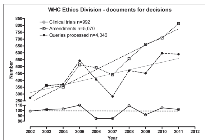
Fig. 3. X-Y plots for the frequency of 'documents for decision' by year.
