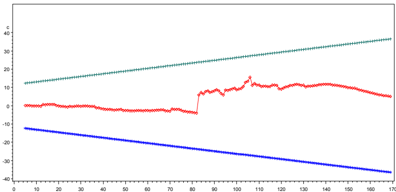
Figure1. CUSUM Test (on Short-run Residuals of the Model)
