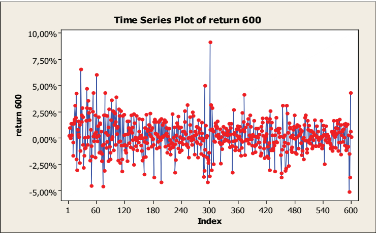
Figure 7. Time Series Plot of JII Return (600 observations) from 2 nd march 2009 to 12 th august 2011
