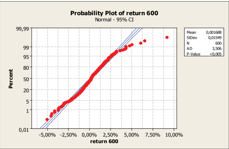
Figure 9. Probability Plot of JII return (600 observations) from 2 nd March 2009 to 12 th August 2011
