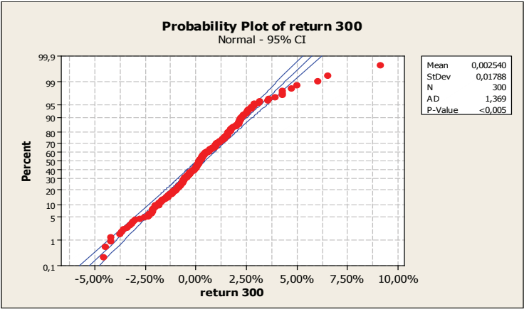
Figure 6. Probability Plot of return of JII (300 observations) from 2 nd march 2009 to 26 th May 2010
