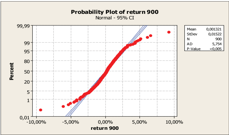
Figure 12. Probability Plot of JII Return (900 observations) from 2 nd March 2009 to 30 th October 2012
