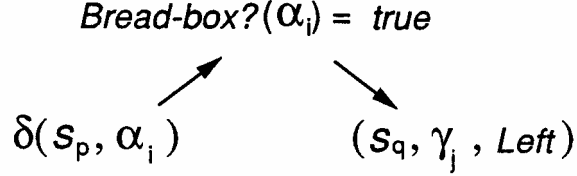
Figure 4: A non-formal \delta transition on symbol \alpha_i . The new machine configuration depends on information about \alpha_i that is not an intrinsic property of the symbol.
